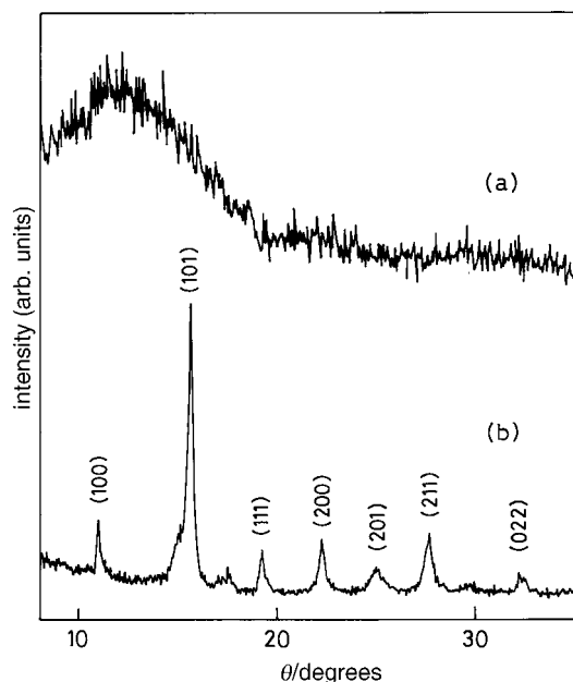
Fig. 10 X-Ray diffraction patterns of PZT powder: (a) as obtained at 723 K, (b) after heating at 823 K for 12 h
