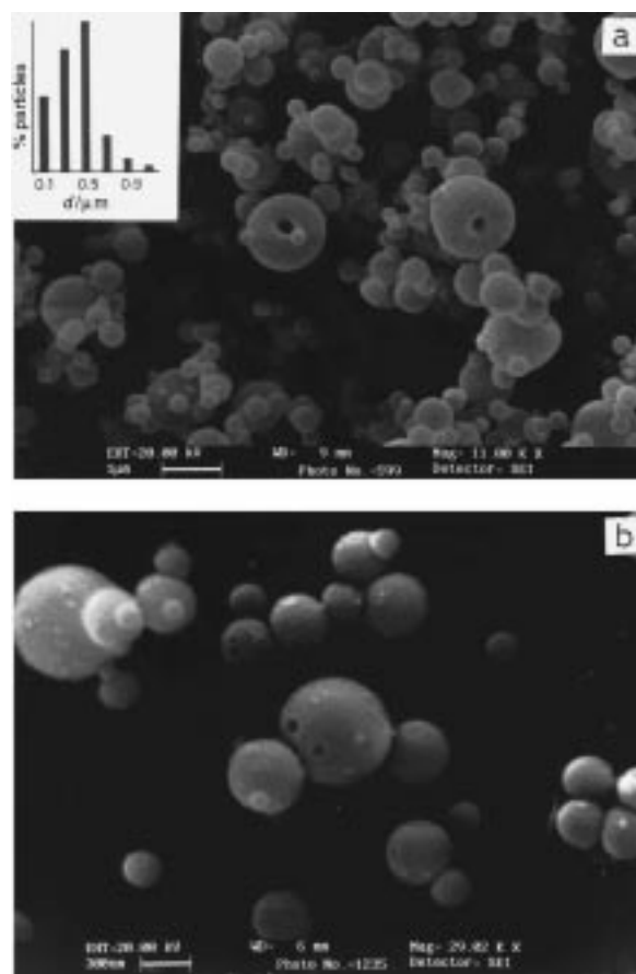
Fig. 2 Scanning electron micrographs of TiO 2 particles: (a) as obtained by nebulized spray pyrolysis at 723 K (the inset shows the particle size distribution of the powder) and (b) after heating the powder at 773 K for 12 h
