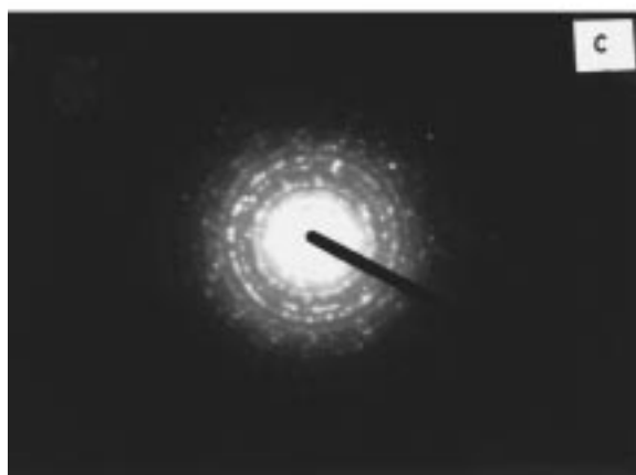
Fig. 3 Transmission electron micrographs of \text{TiO}_2 particles: (a) as obtained by nebulized spray pyrolysis at 723 K, (b) after heating the powder at 773 K for 12 h and (c) electron diffraction pattern of the powder heated at 773 K for 12 h
